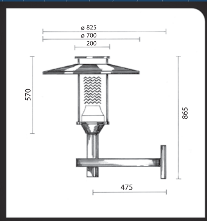
W-5500 Wandarm
